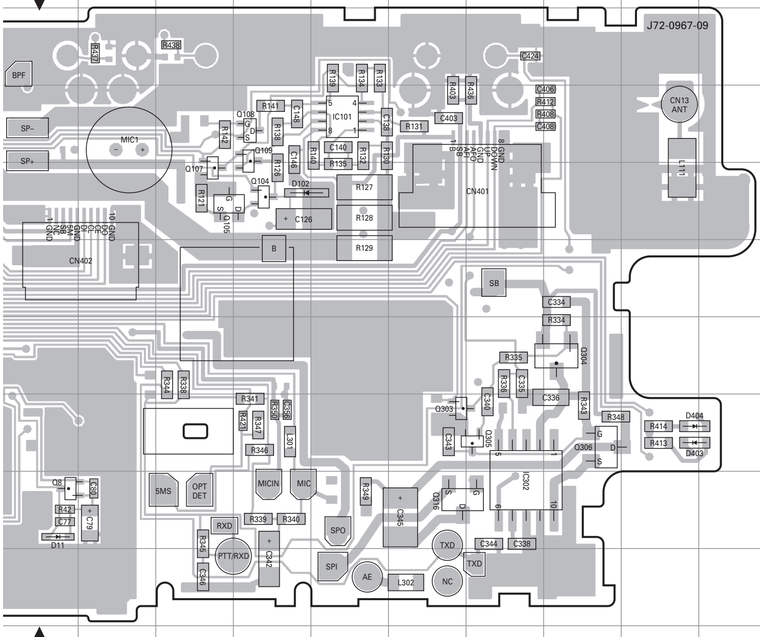
TX-RX UNIT (X57-7120-XX) Component side view (J72-0967-09) -10 : TK-2212 (K,M), TK-2217 (M) -21 : TK-2217 (M3)
